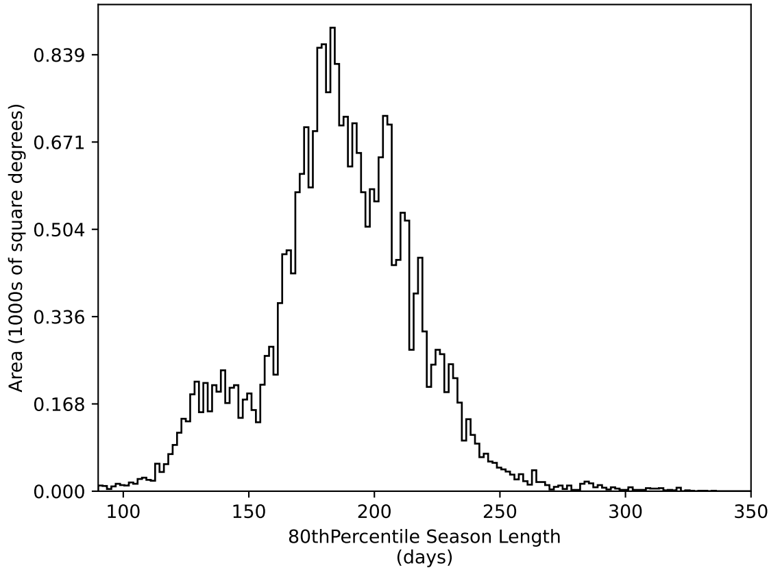
too_elab_r64_d2_ugrizy_v3.4_10yrs All sky all bands: 80thPercentile Season Length
