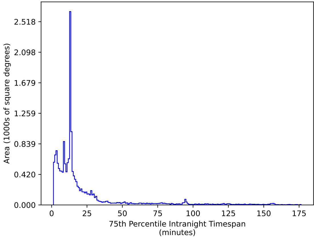
too_elab_r64_d2_ugrizy_v3.4_10yrs WFD z band: 75th Percentile Intranight Timespan
