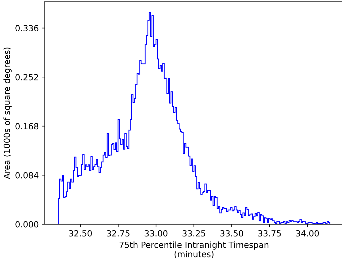
too_elab_r64_d2_ugrizy_v3.4_10yrs WFD y band: 75th Percentile Intranight Timespan
