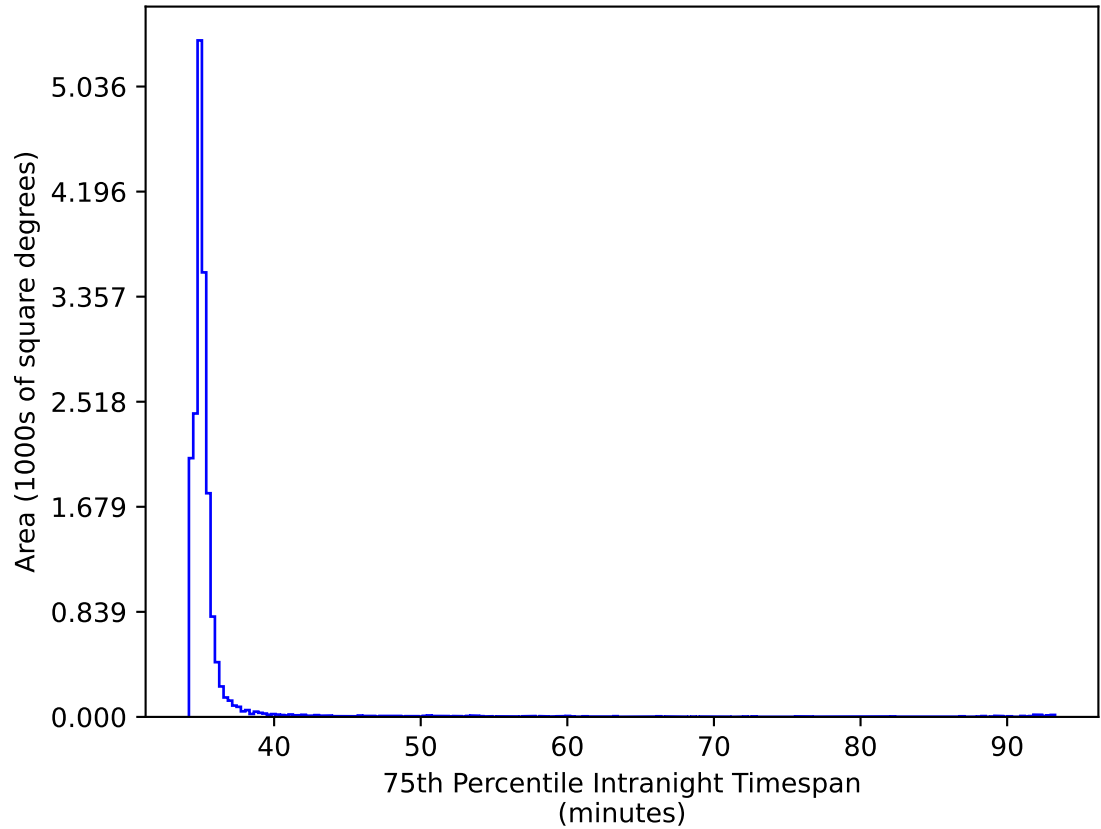
too_elab_r64_d2_ugrizy_v3.4_10yrs WFD ri bands: 75th Percentile Intranight Timespan
