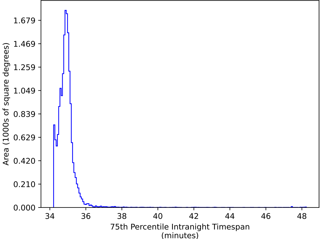
too_elab_r64_d2_ugrizy_v3.4_10yrs WFD iz bands: 75th Percentile Intranight Timespan
