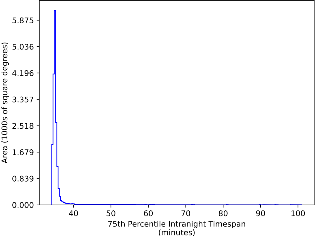
too_elab_r64_d2_ugrizy_v3.4_10yrs WFD gr bands: 75th Percentile Intranight Timespan
