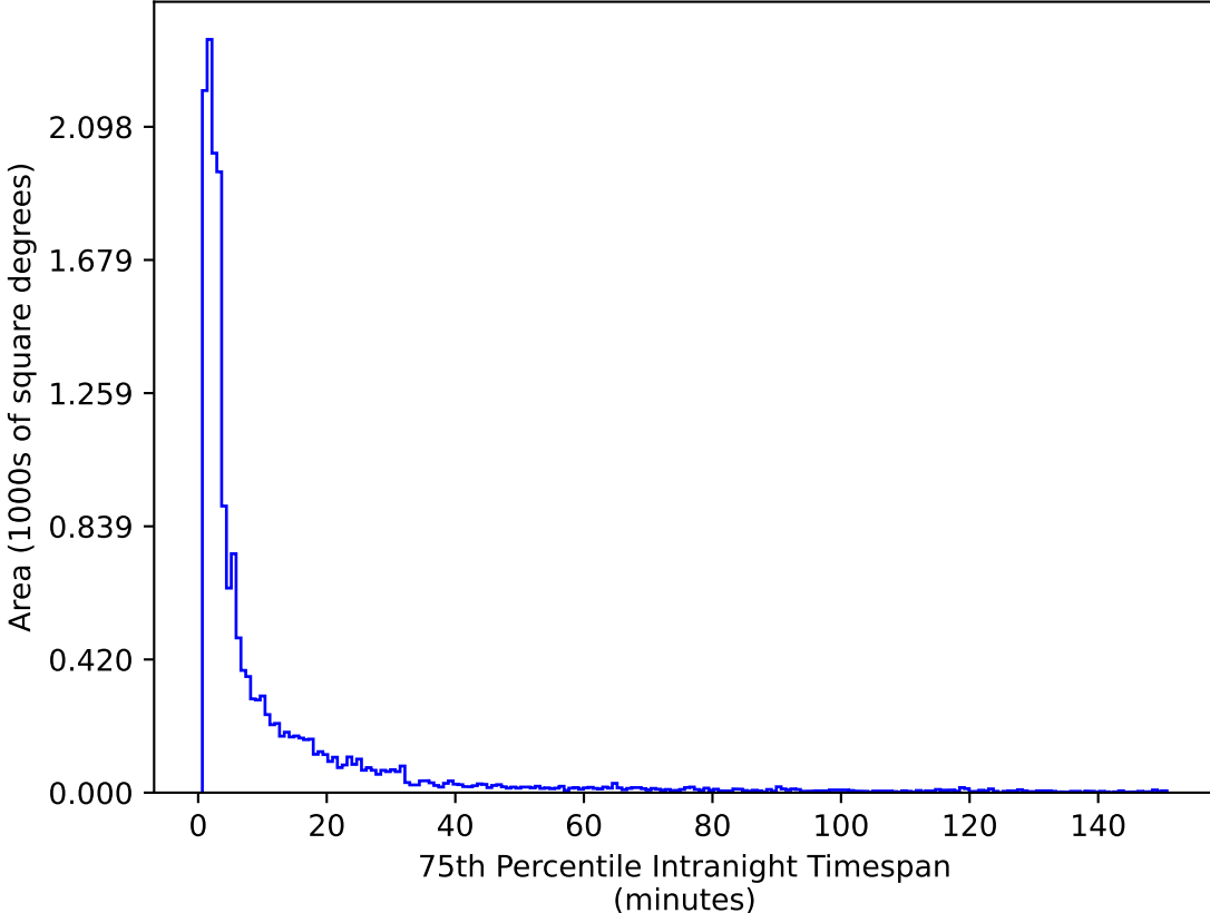
too_elab_r64_d2_ugrizy_v3.4_10yrs WFD g band: 75th Percentile Intranight Timespan
