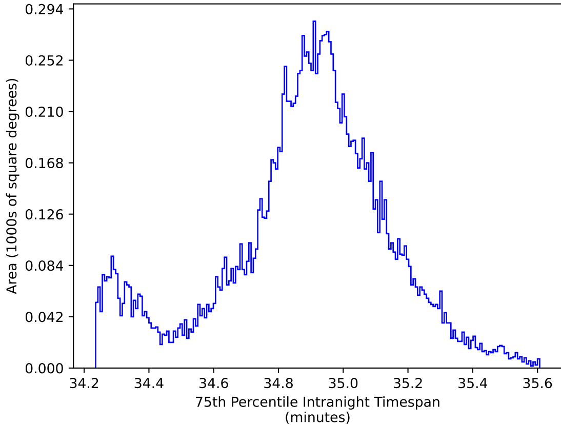
too_elab_r64_d2_ugrizy_v3.4_10yrs WFD all bands: 75th Percentile Intranight Timespan
