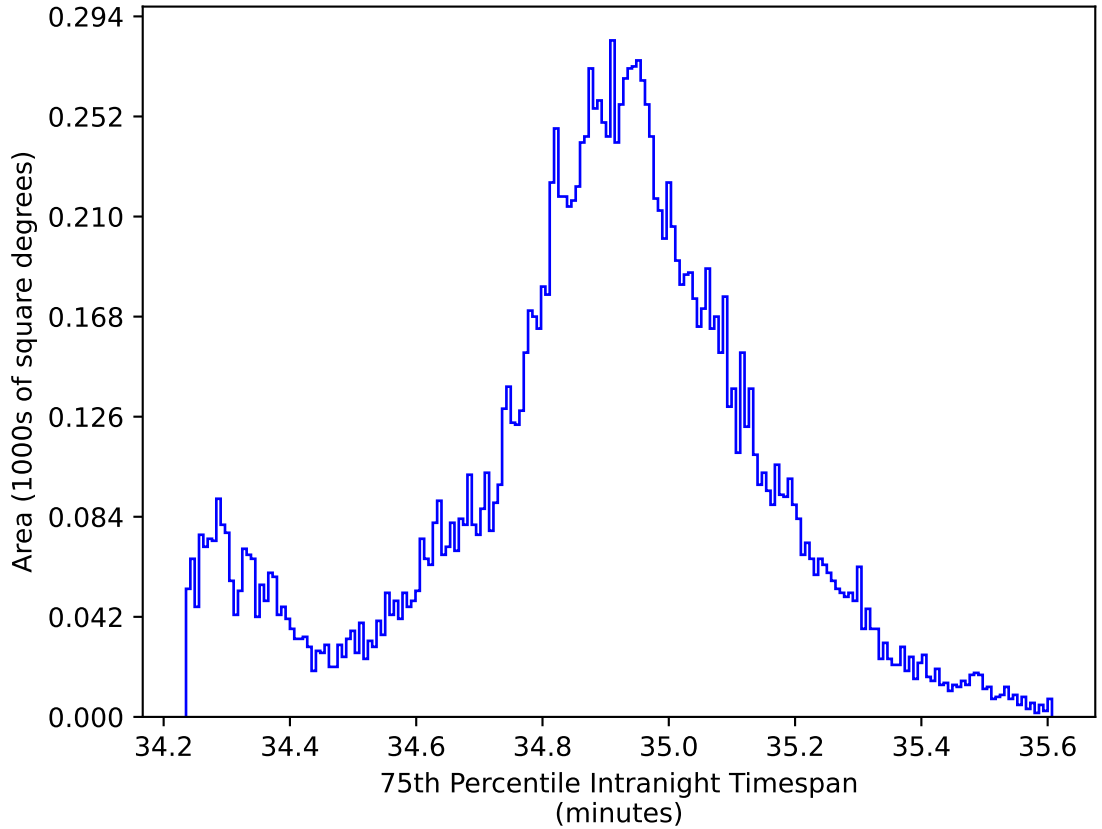
too_elab_r64_d2_ugrizy_v3.4_10yrs WFD: 75th Percentile Intranight Timespan
