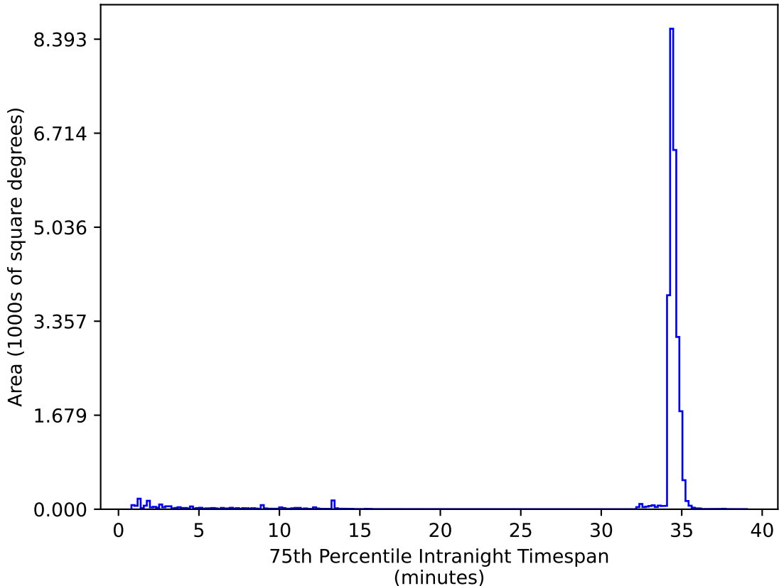
too_elab_r64_d2_ugrizy_v3.4_10yrs All sky zy bands: 75th Percentile Intranight Timespan
