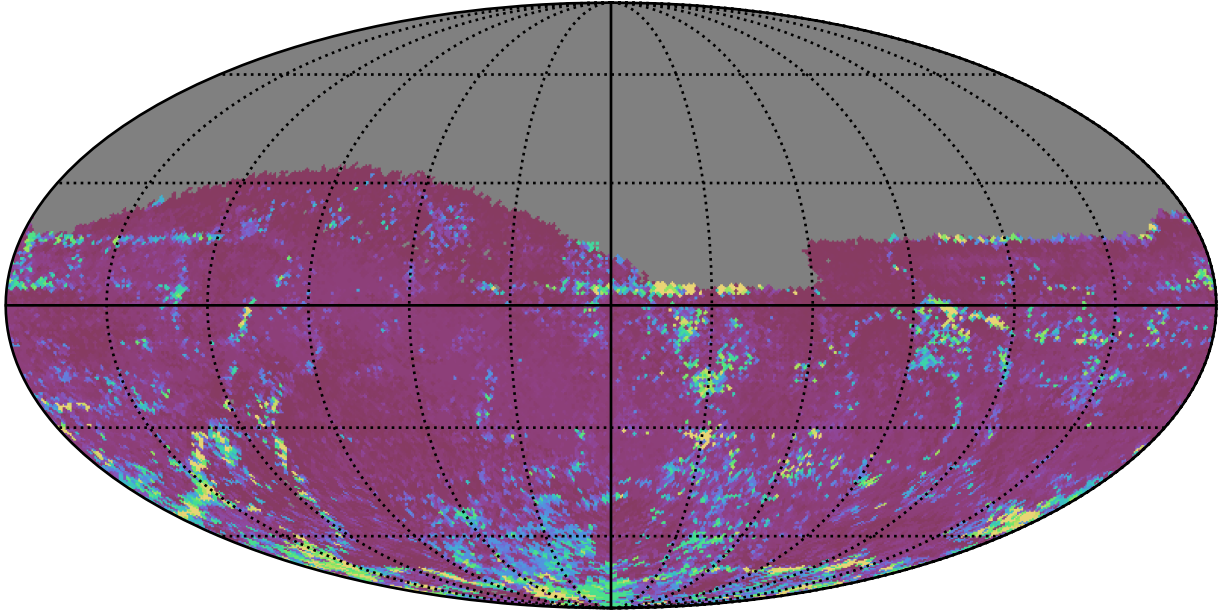
too_elab_r64_d2_ugrizy_v3.4_10yrs All sky z band: 75th Percentile Intranight Timespan
