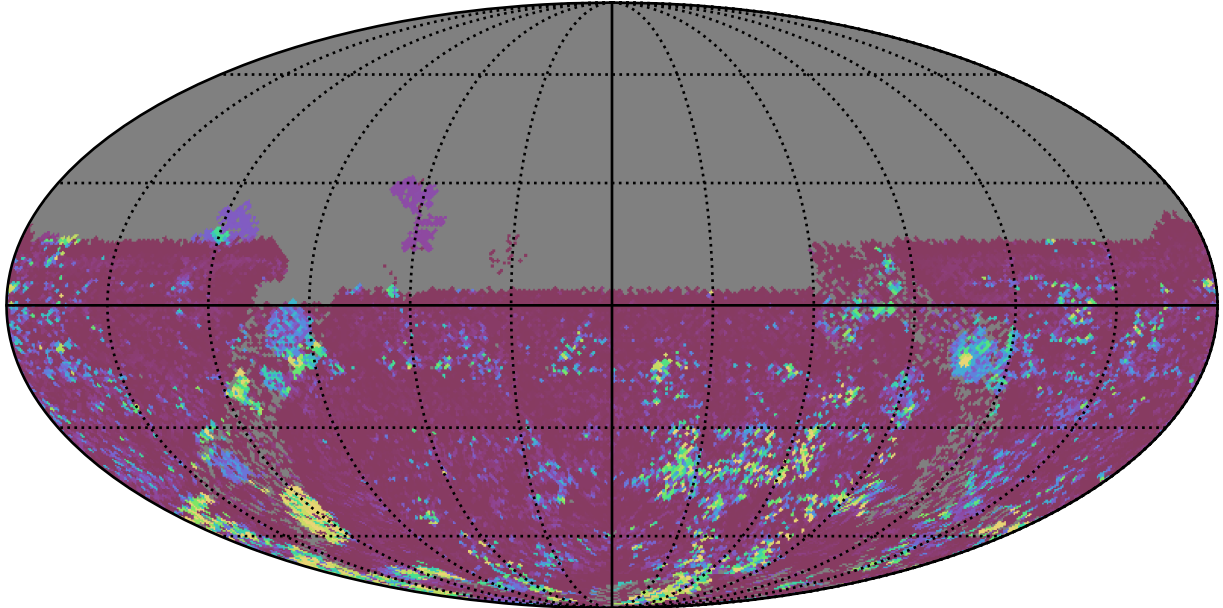
too_elab_r64_d2_ugrizy_v3.4_10yrs All sky u band: 75th Percentile Intranight Timespan
