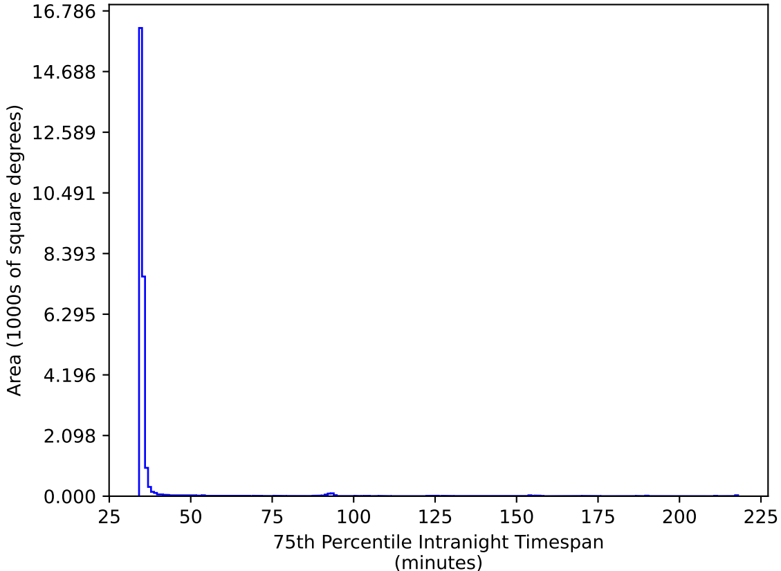
too_elab_r64_d2_ugrizy_v3.4_10yrs All sky ri bands: 75th Percentile Intranight Timespan
