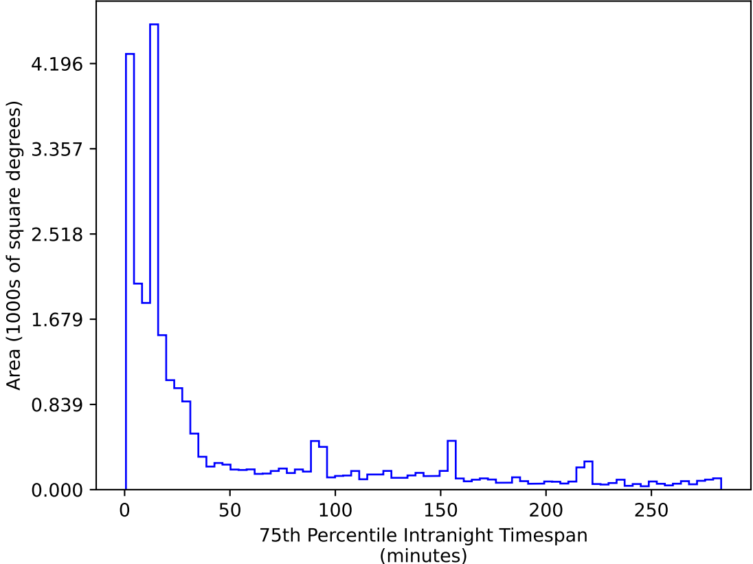
too_elab_r64_d2_ugrizy_v3.4_10yrs All sky r band: 75th Percentile Intranight Timespan
