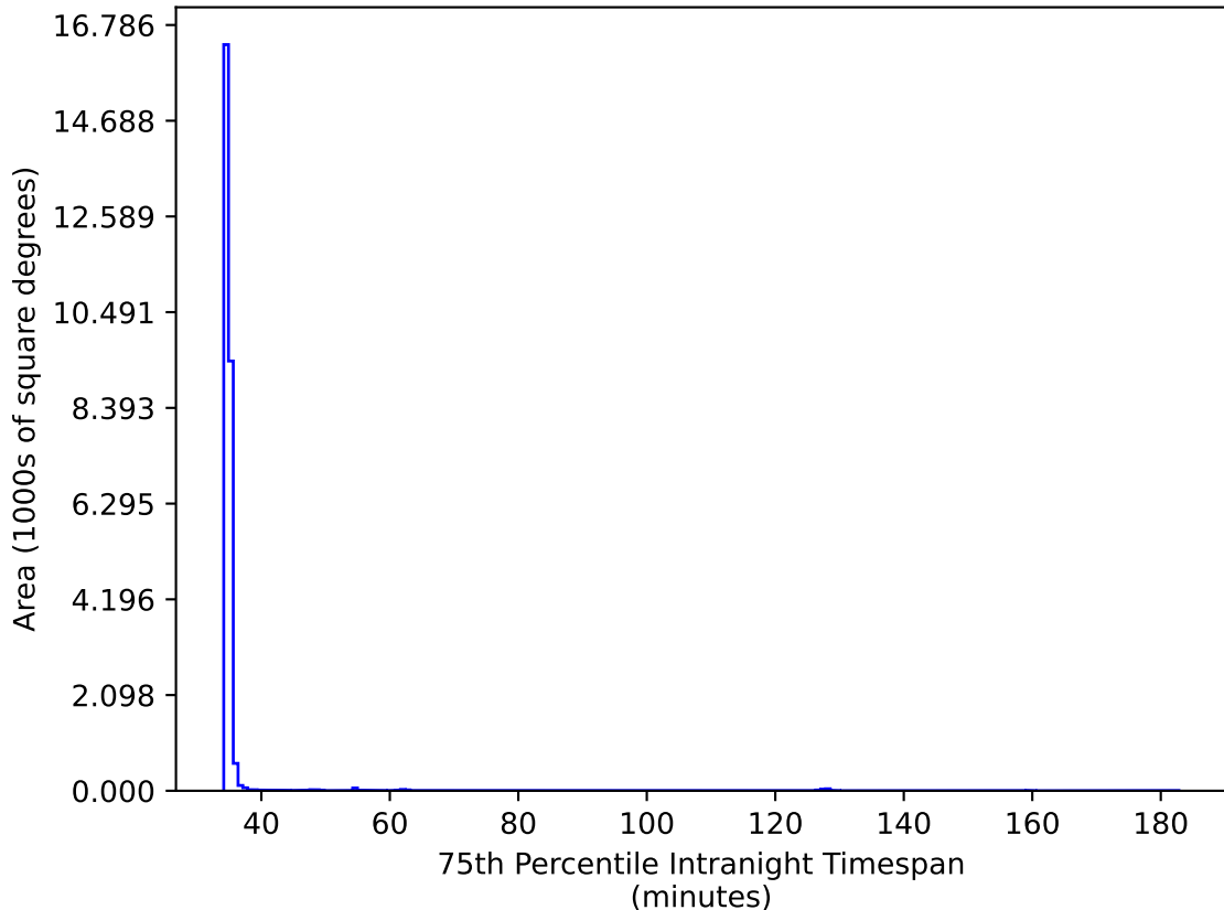
too_elab_r64_d2_ugrizy_v3.4_10yrs All sky iz bands: 75th Percentile Intranight Timespan
