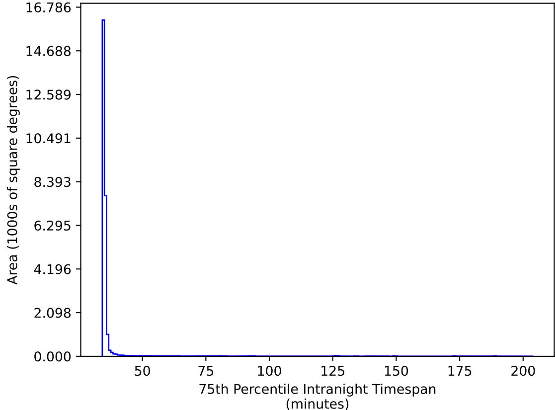
too_elab_r64_d2_ugrizy_v3.4_10yrs All sky gr bands: 75th Percentile Intranight Timespan
