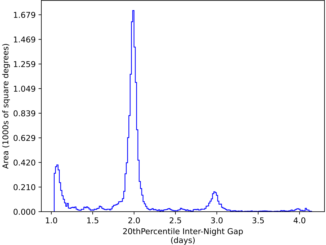
too_elab_r64_d2_ugrizy_v3.4_10yrs WFD y band: 20thPercentile Inter-Night Gap
