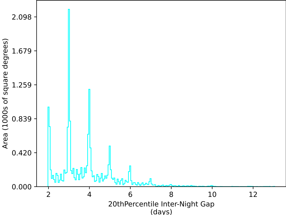
too_elab_r64_d2_ugrizy_v3.4_10yrs WFD u band: 20thPercentile Inter-Night Gap
