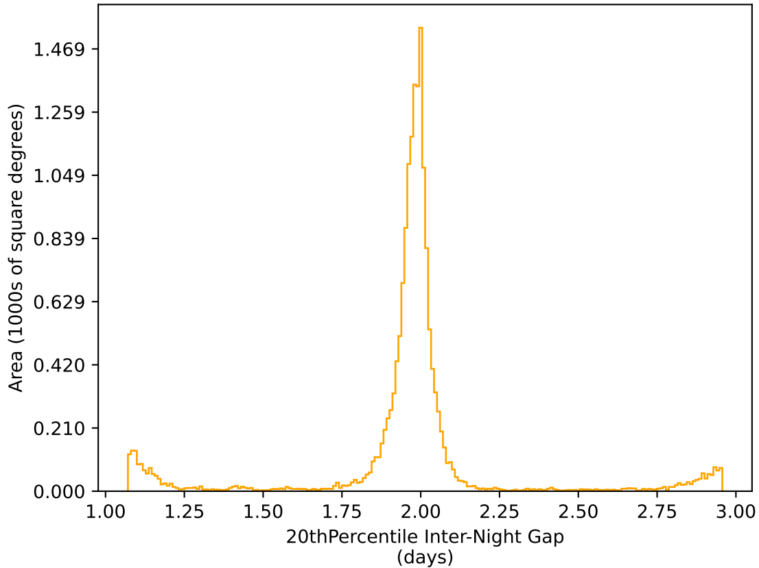
too_elab_r64_d2_ugrizy_v3.4_10yrs WFD r band: 20thPercentile Inter-Night Gap
