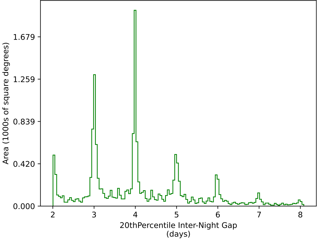
too_elab_r64_d2_ugrizy_v3.4_10yrs WFD g band: 20thPercentile Inter-Night Gap
