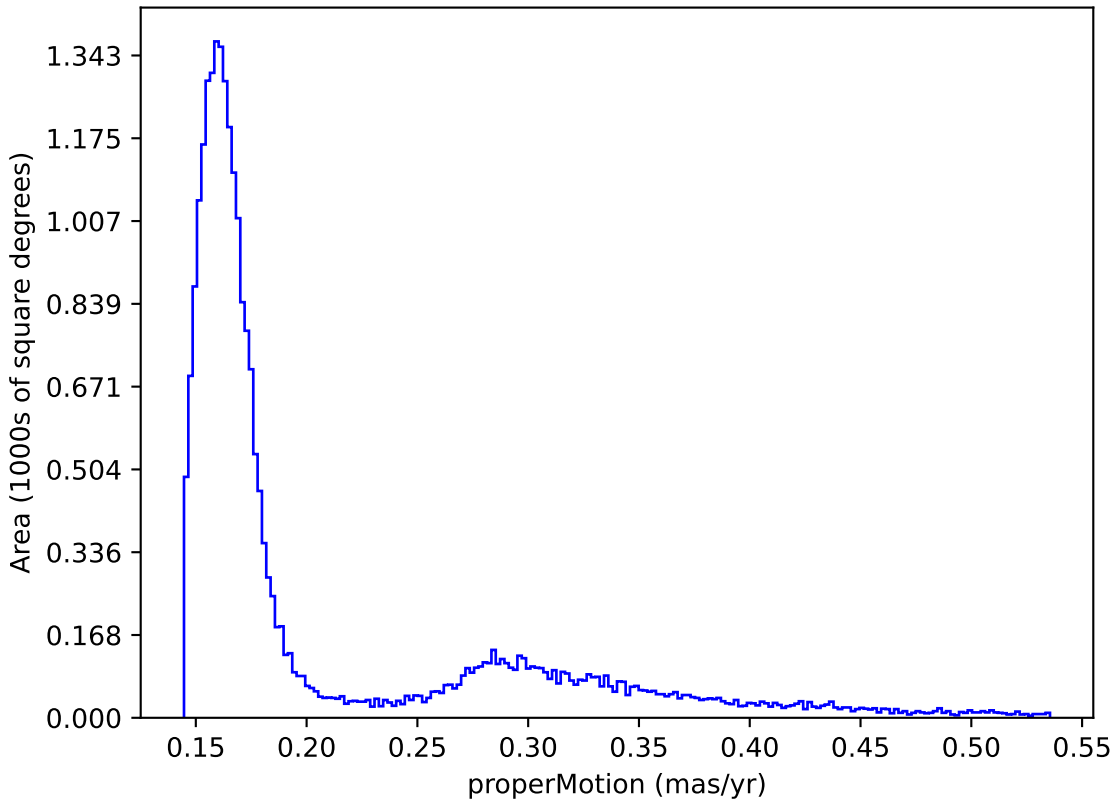
too_elab_r64_d2_ugrizy_v3.4_10yrs : properMotion
