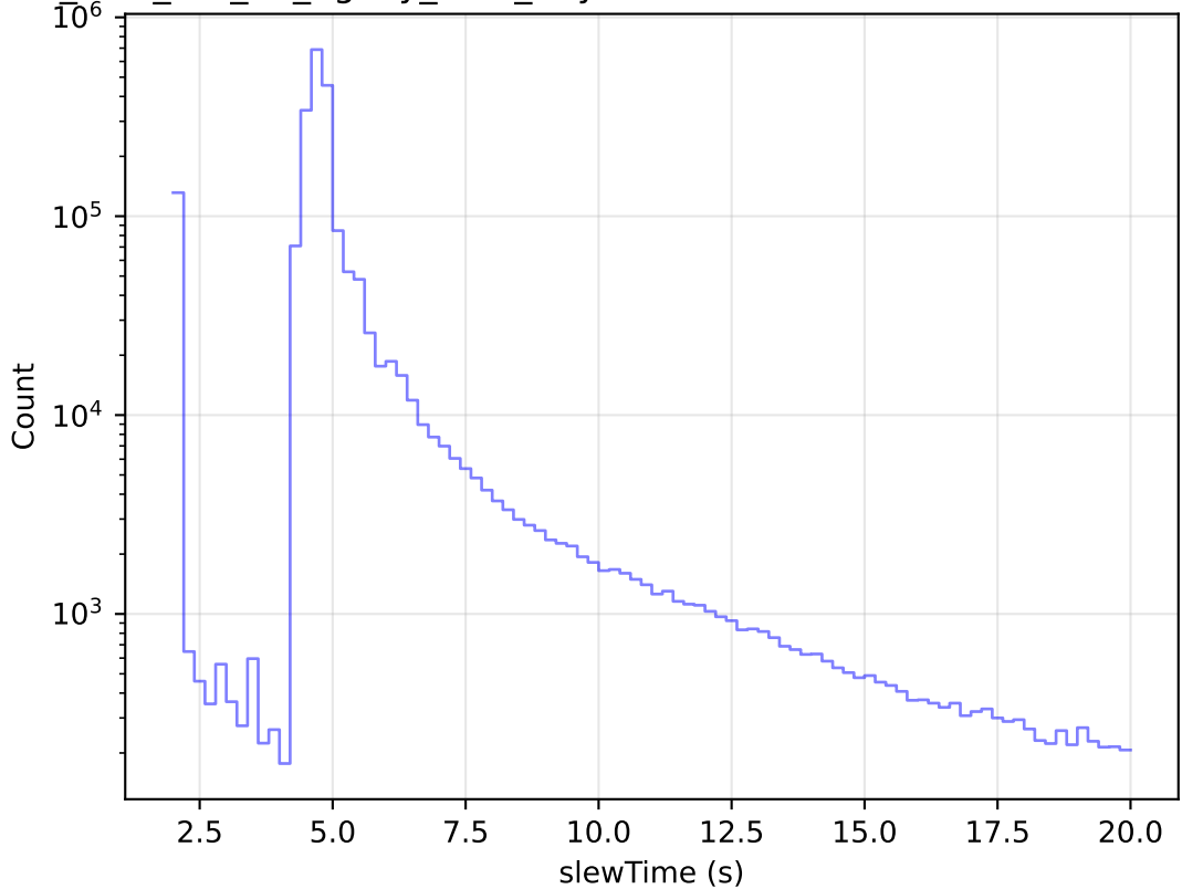
too_elab_r64_d2_ugrizy_v3.4_10yrs All visits: Zoom Slew Time Histogram
