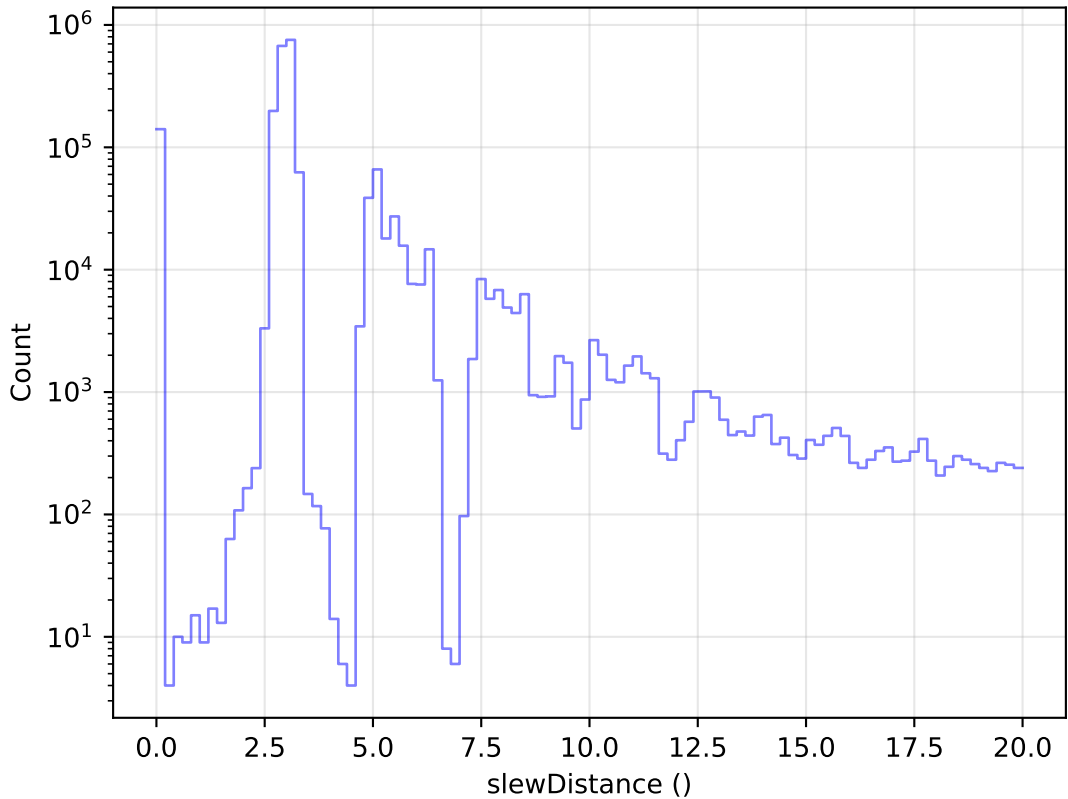
too_elab_r64_d2_ugrizy_v3.4_10yrs All visits: Zoom Slew Distance Histogram
