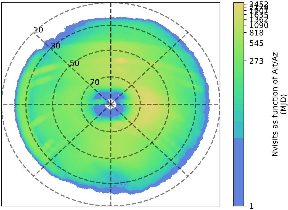
too_elab_r64_d2_ugrizy_v3.4_10yrs r: Nvisits as function of Alt/Az
