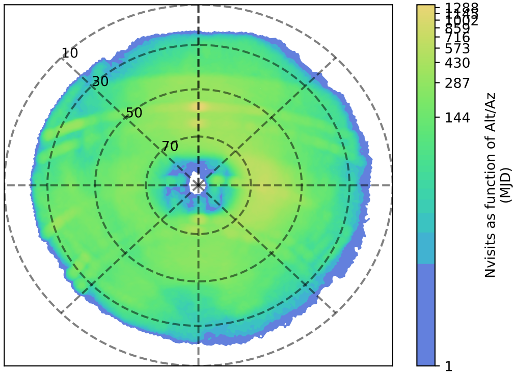
too_elab_r64_d2_ugrizy_v3.4_10yrs g: Nvisits as function of Alt/Az
