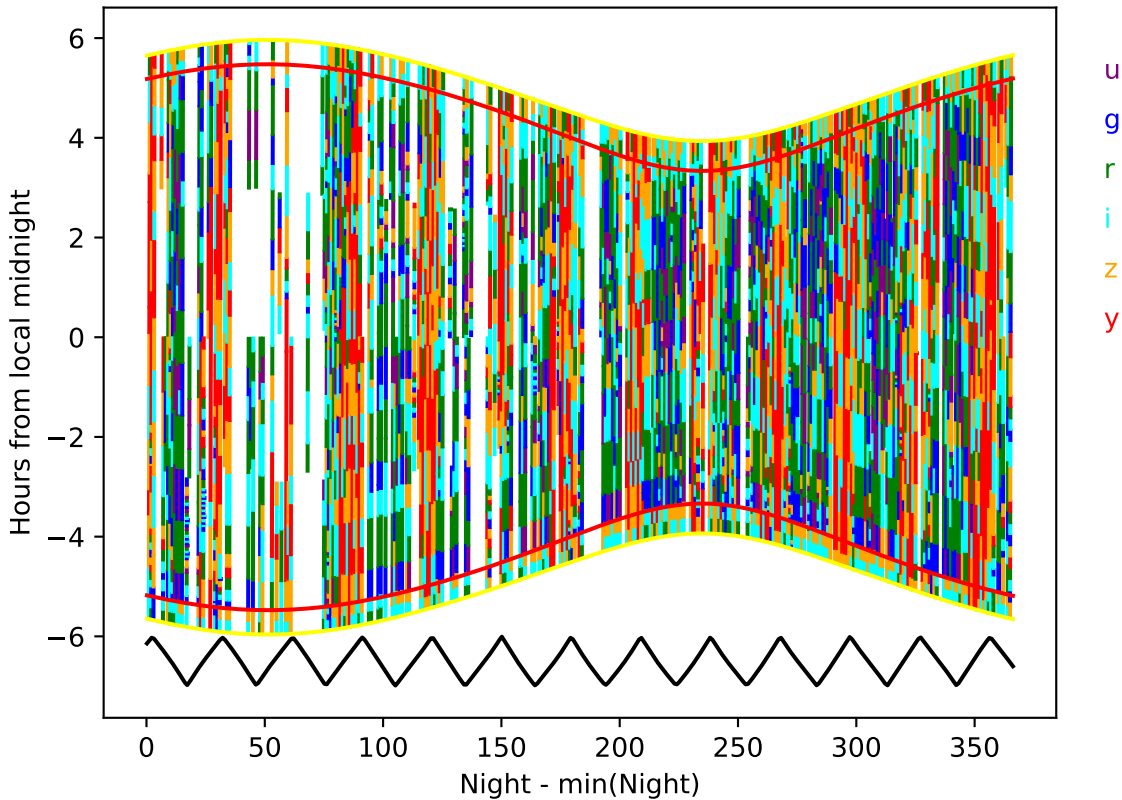
too_elab_r64_d2_ugrizy_v3.4_10yrs year 9-10: Hourglass
