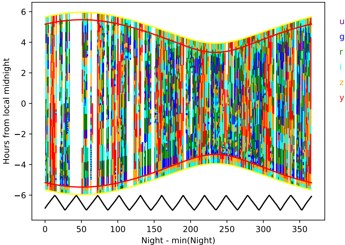
too_elab_r64_d2_ugrizy_v3.4_10yrs year 8-9: Hourglass
