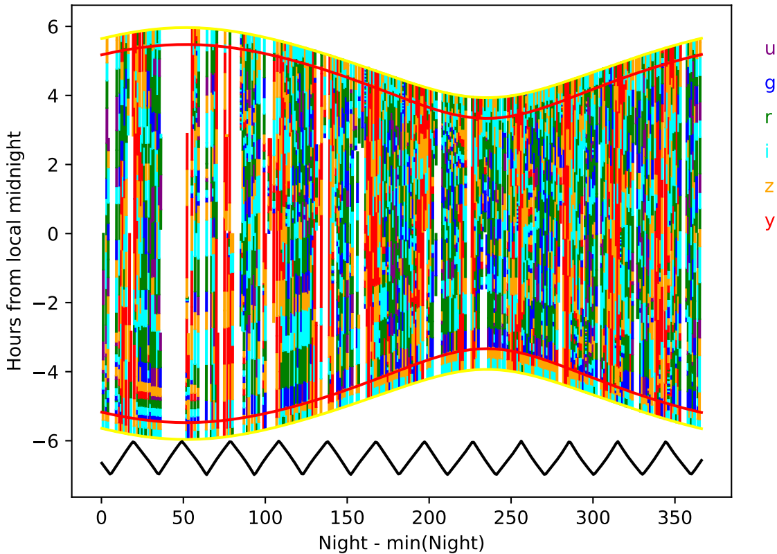
too_elab_r64_d2_ugrizy_v3.4_10yrs year 2-3: Hourglass
