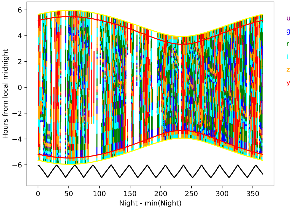
too_elab_r64_d2_ugrizy_v3.4_10yrs year 1-2: Hourglass
