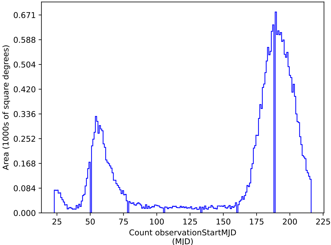
too_elab_r64_d2_ugrizy_v3.4_10yrs i: Count observationStartMJD
