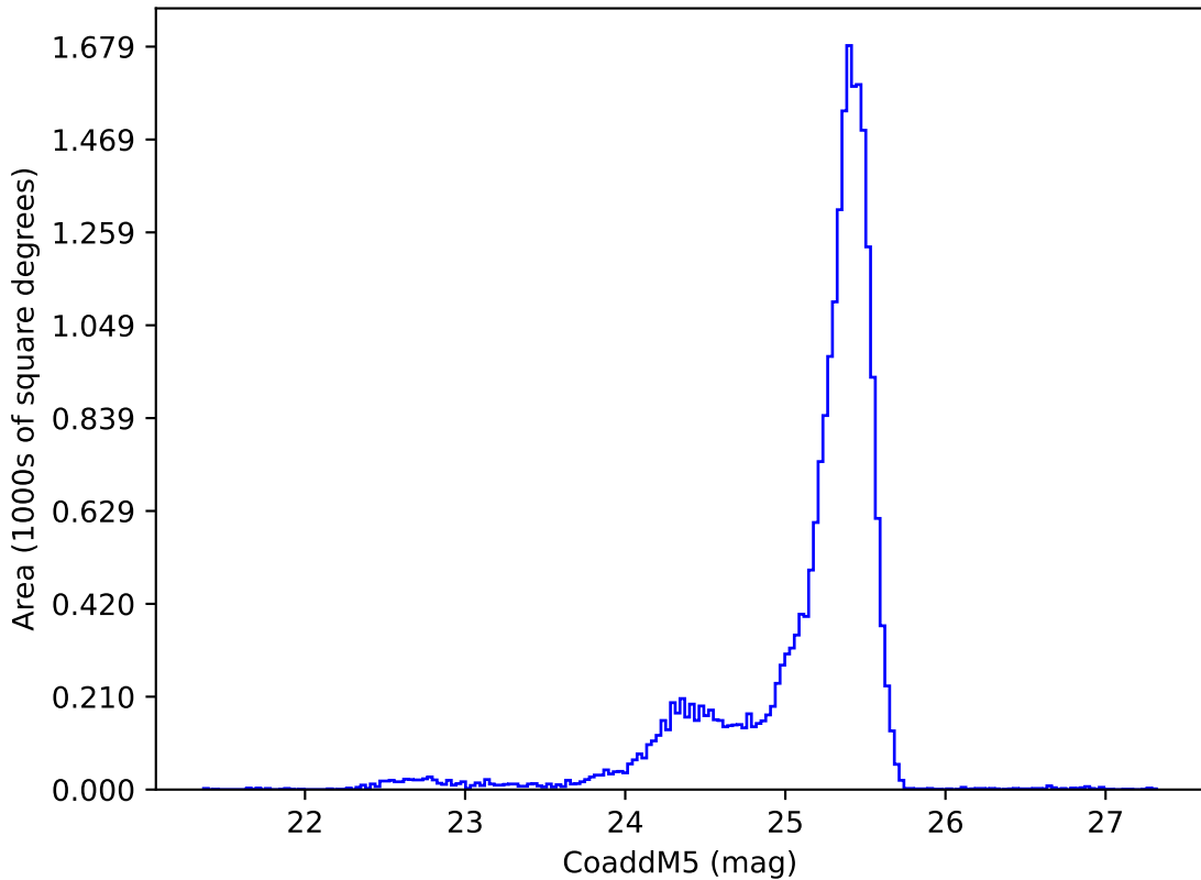
too_elab_r64_d2_ugrizy_v3.4_10yrs u: CoaddM5
