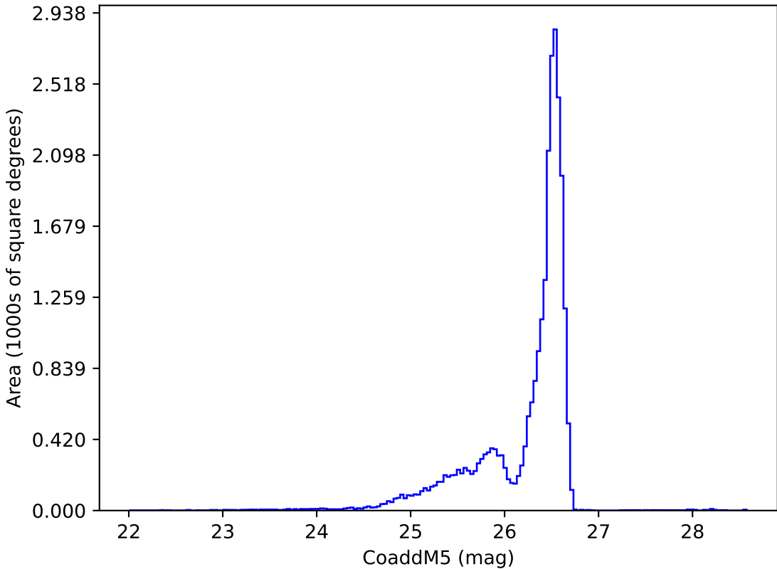
too_elab_r64_d2_ugrizy_v3.4_10yrs i: CoaddM5
