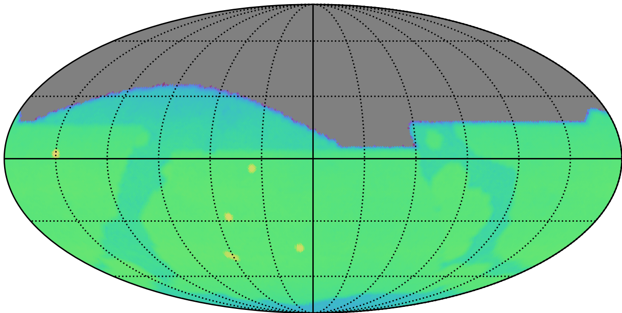
too_elab_r64_d2_ugrizy_v3.4_10yrs : CoaddM5
