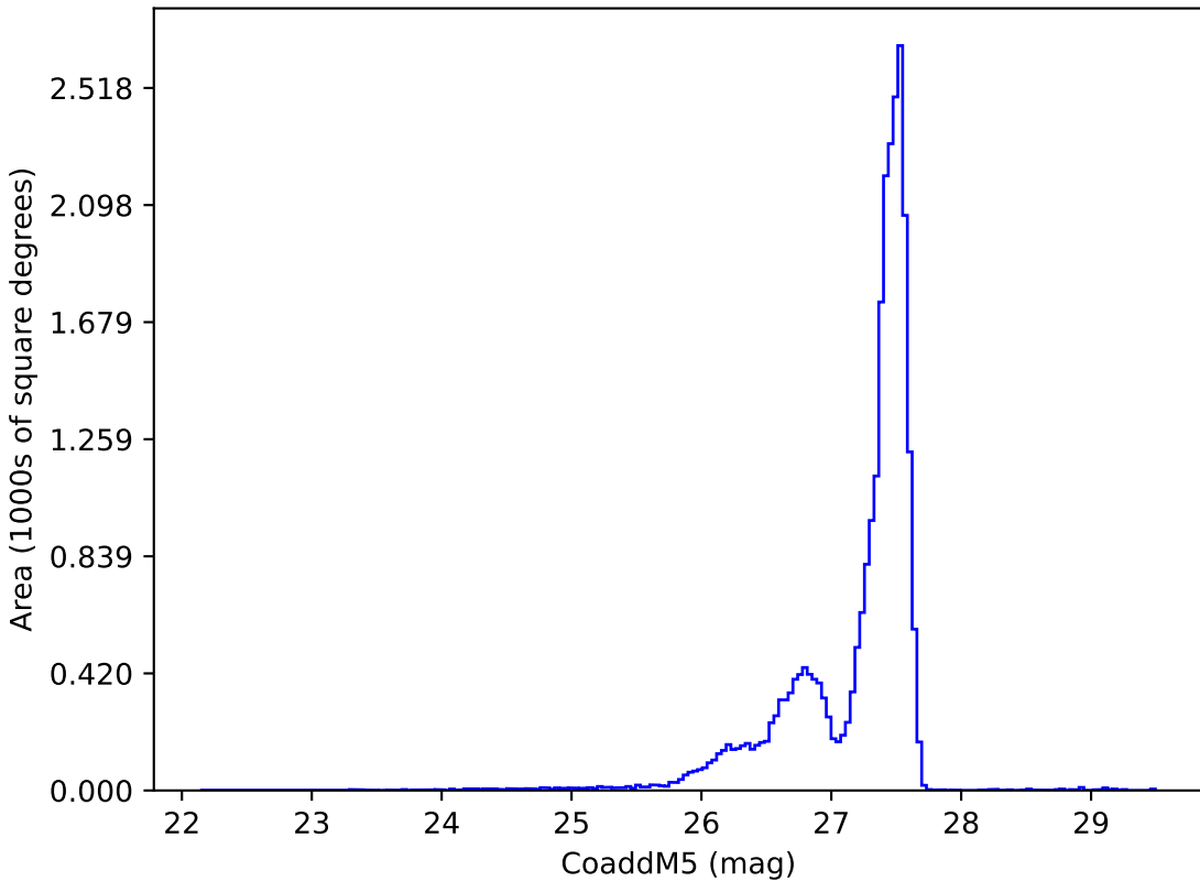
too_elab_r64_d2_ugrizy_v3.4_10yrs : CoaddM5
