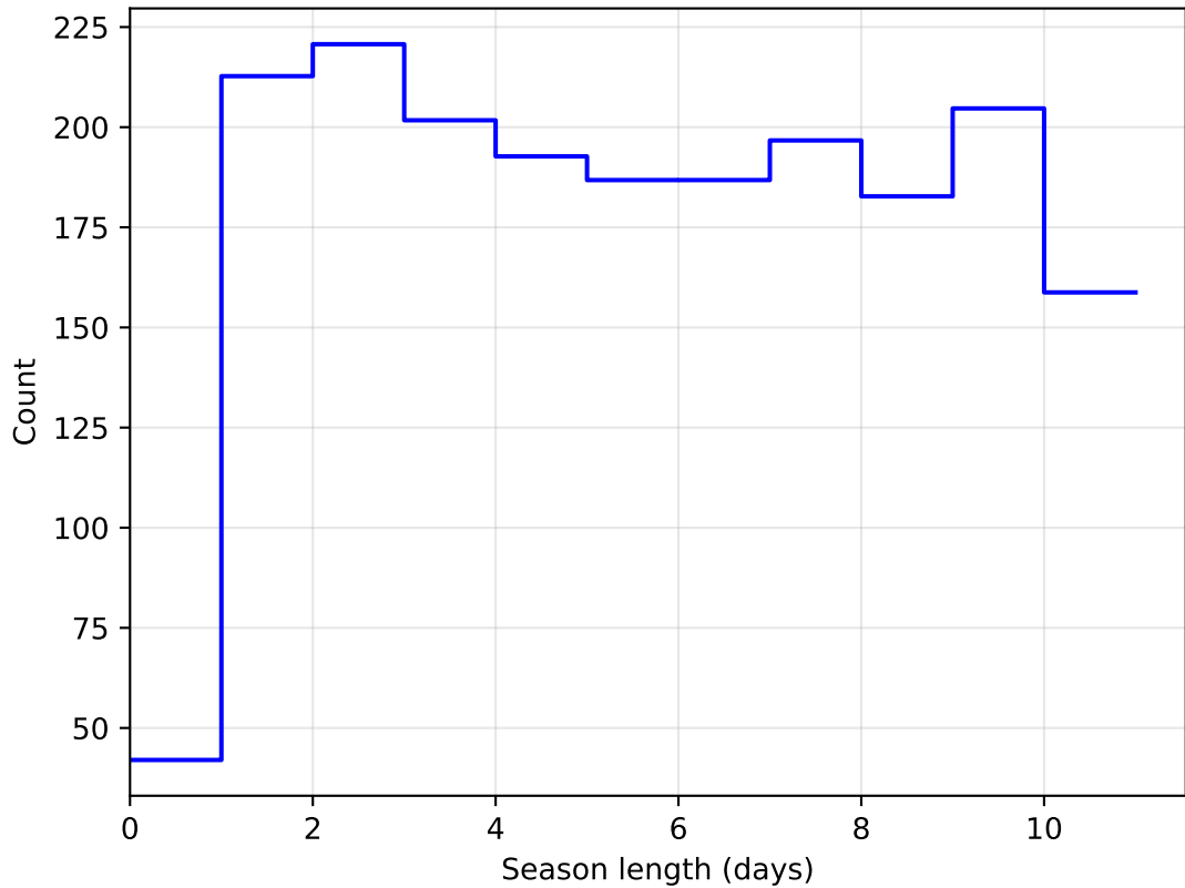
too_elab_r64_d2_ugrizy_v3.4_10yrs DD: COSMOS all bands: SeasonLength
