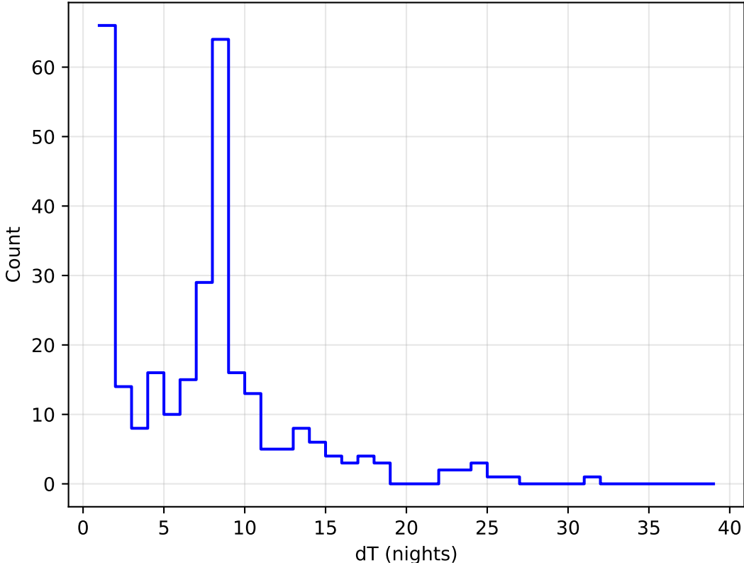
too_elab_r64_d2_ugrizy_v3.4_10yrs all bands: DD:XMM_LSS Delta Nights Histogram
