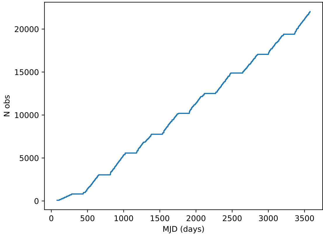
too_elab_r64_d2_ugrizy_v3.4_10yrs all bands: DD:XMM_LSS Cumulative NVisits
