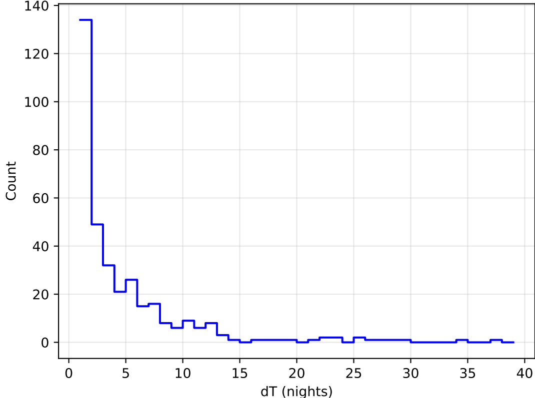
too_elab_r64_d2_ugrizy_v3.4_10yrs all bands: DD:WFD Delta Nights Histogram
