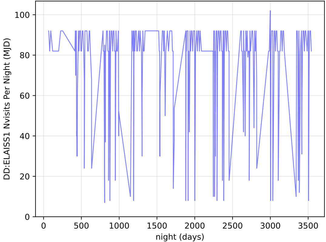
too_elab_r64_d2_ugrizy_v3.4_10yrs all bands: DD:ELAISS1 Nvisits Per Night
