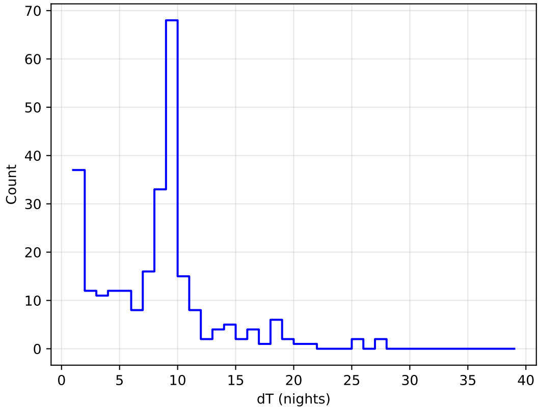
too_elab_r64_d2_ugrizy_v3.4_10yrs all bands: DD:ELAISS1 Delta Nights Histogram
