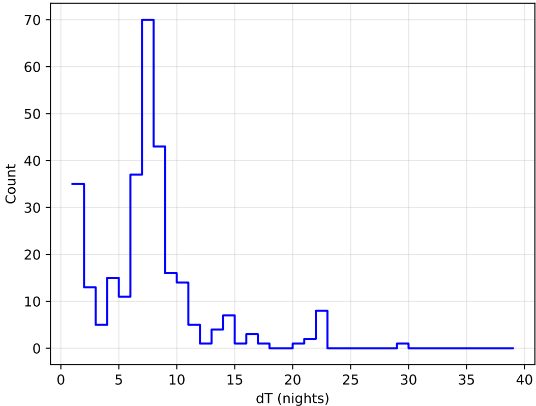
too_elab_r64_d2_ugrizy_v3.4_10yrs all bands: DD:EDFS Delta Nights Histogram
