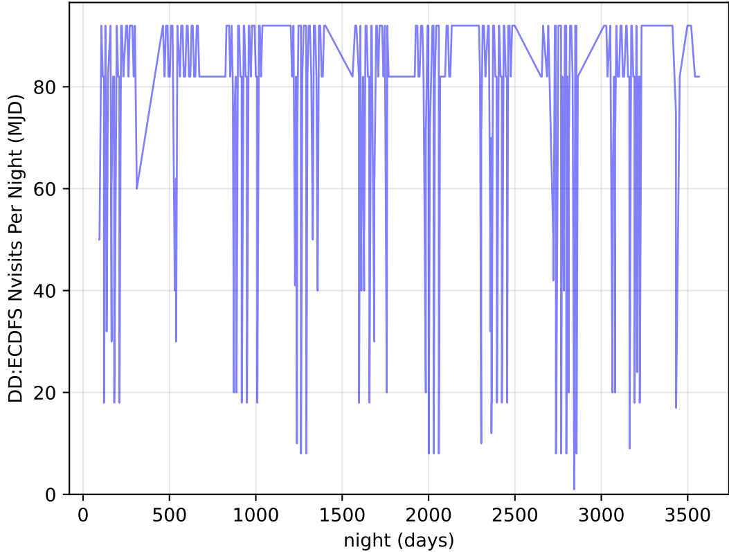
too_elab_r64_d2_ugrizy_v3.4_10yrs all bands: DD:ECDFS Nvisits Per Night
