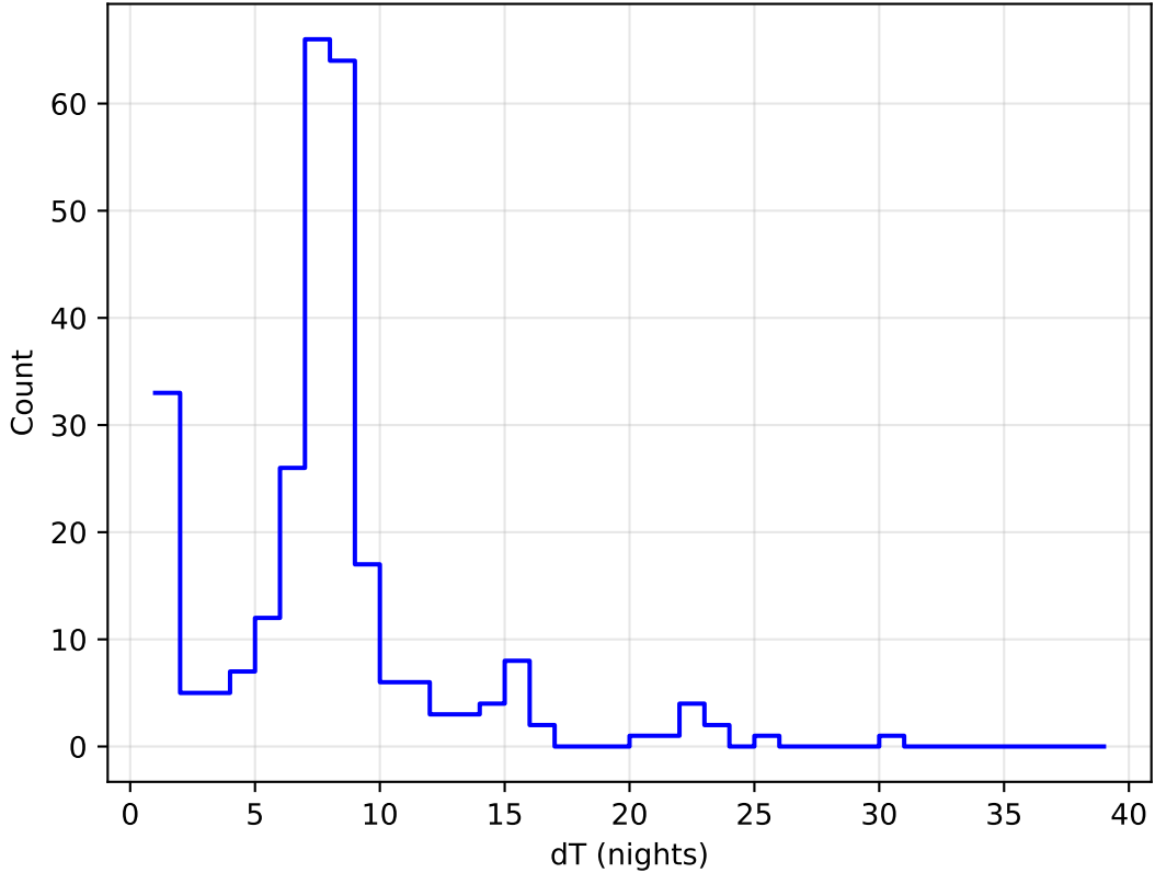
too_elab_r64_d2_ugrizy_v3.4_10yrs all bands: DD:ECDFS Delta Nights Histogram
