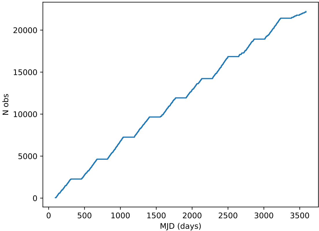
too_elab_r64_d2_ugrizy_v3.4_10yrs all bands: DD:ECDFS Cumulative NVisits
