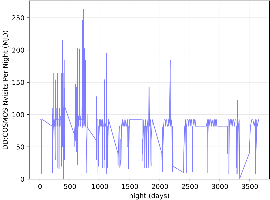
too_elab_r64_d2_ugrizy_v3.4_10yrs all bands: DD: COSMOS Nvisits Per Night
