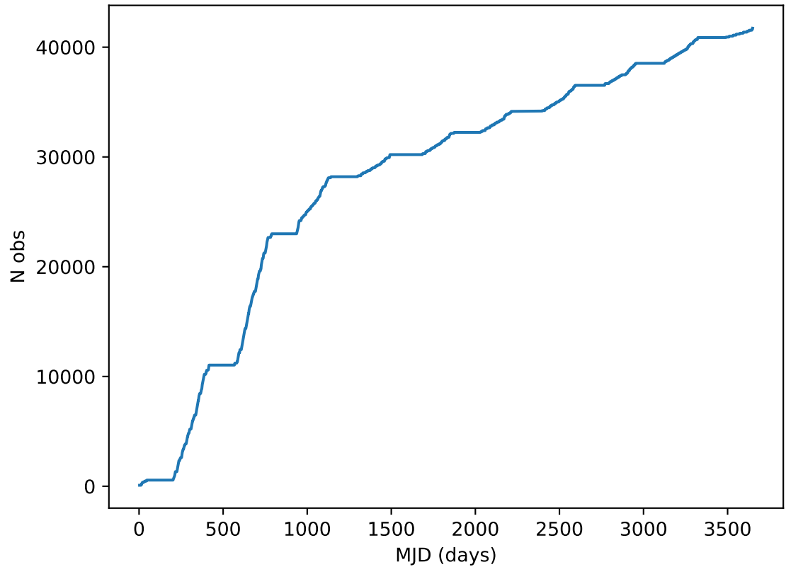
too_elab_r64_d2_ugrizy_v3.4_10yrs all bands: DD: COSMOS Cumulative NVisits
