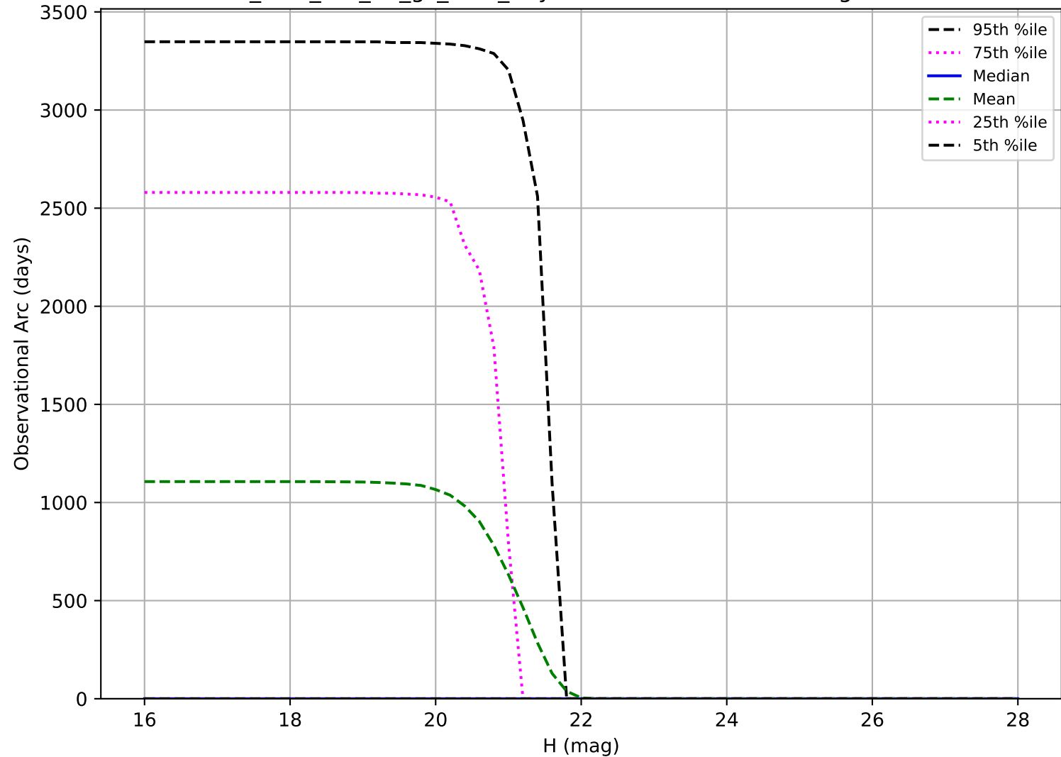
too_elab_r64_d2_gz_v3.4_10yrs: Observational Arc Length Vatra
