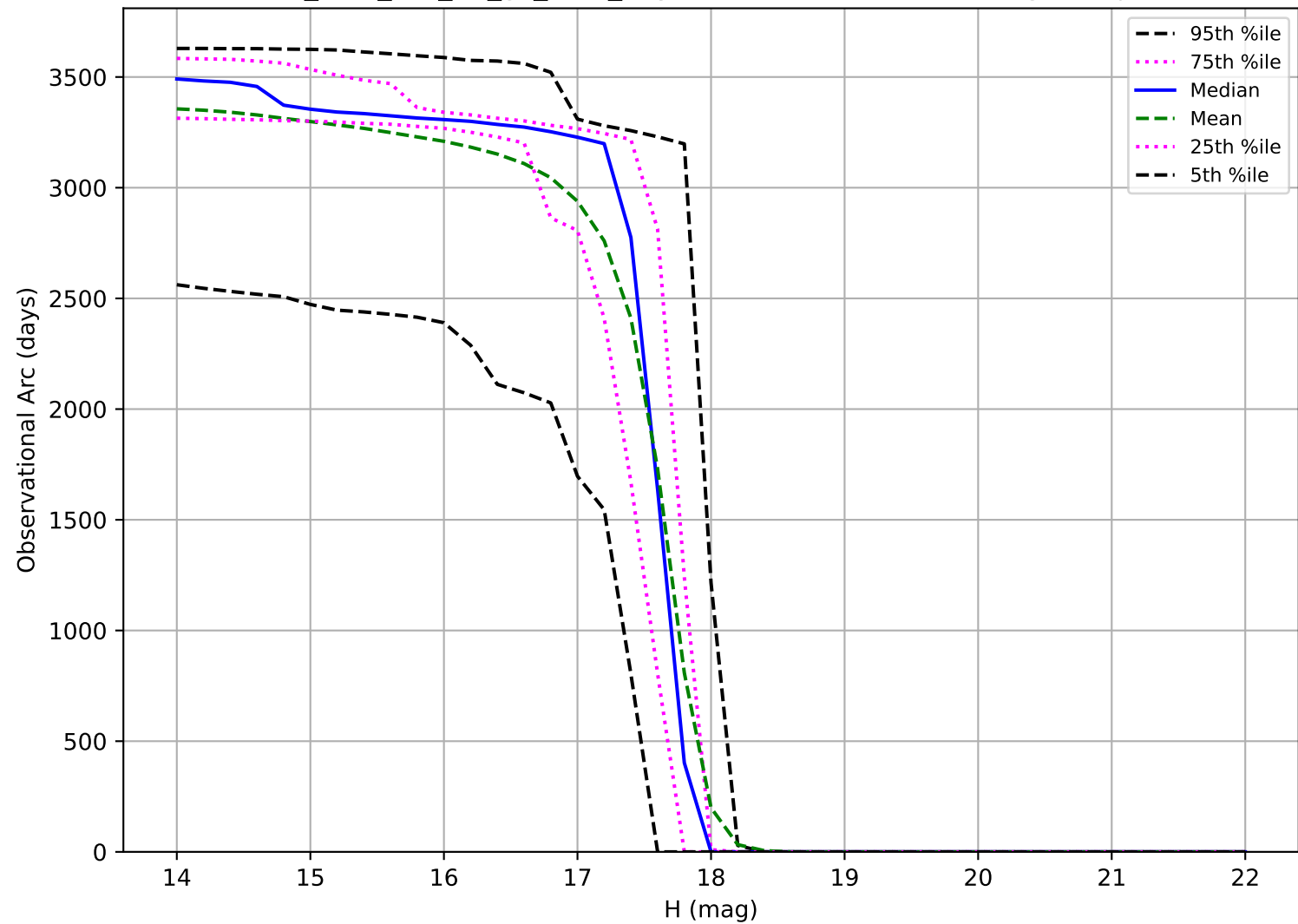
too_elab_r64_d2_gz_v3.4_10yrs: Observational Arc Length Trojan
