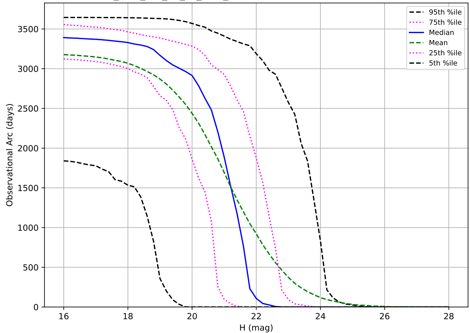
too_elab_r64_d2_gz_v3.4_10yrs: Observational Arc Length NEO
