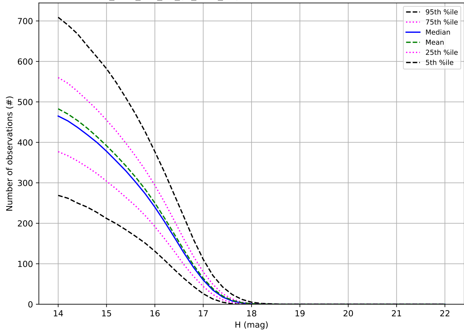
too_elab_r64_d2_gz_v3.4_10yrs: Number of observations Trojan
